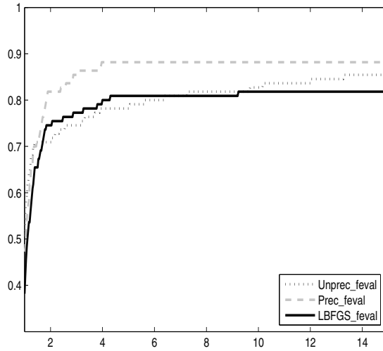
Figure 3 – Comparison of the FR algorithms in terms of number of function evaluations.
