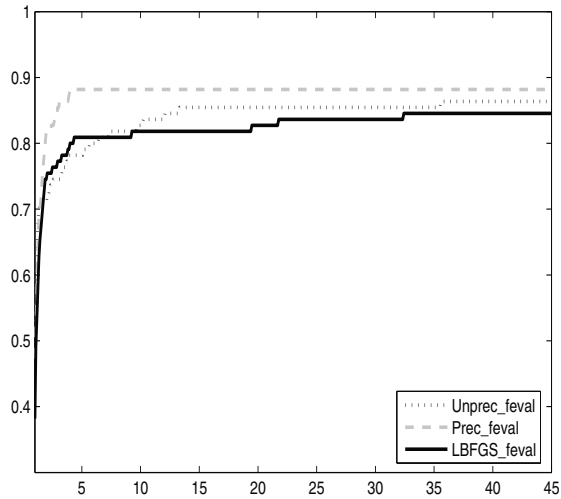
Figure 4 – Comparison of the FR algorithms in terms of number of function evaluations (expanded).
