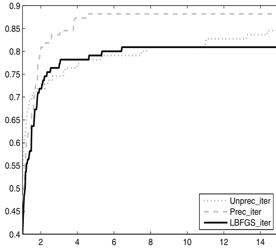
Figure 1 – Comparison of the FR algorithms in terms of number of iterations.
