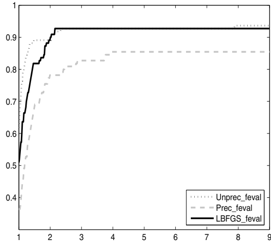
Figure 7 – Comparison of the PR algorithms in terms of number of function evaluations.
