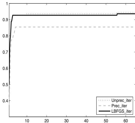
Figure 6 – Comparison of the PR algorithms in terms of number of iterations (expanded).
