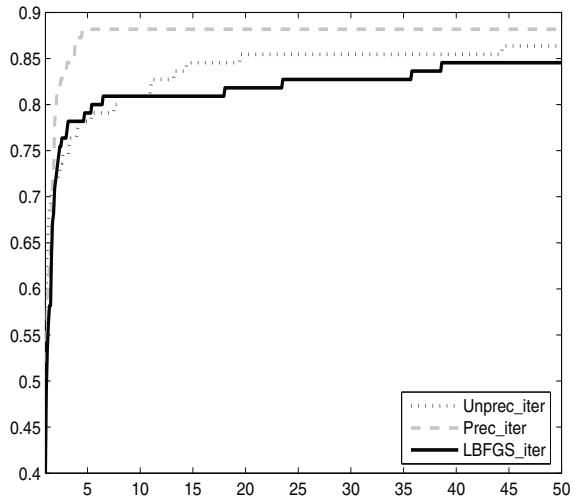
Figure 2 – Comparison of the FR algorithms in terms of number of iterations (expanded).
