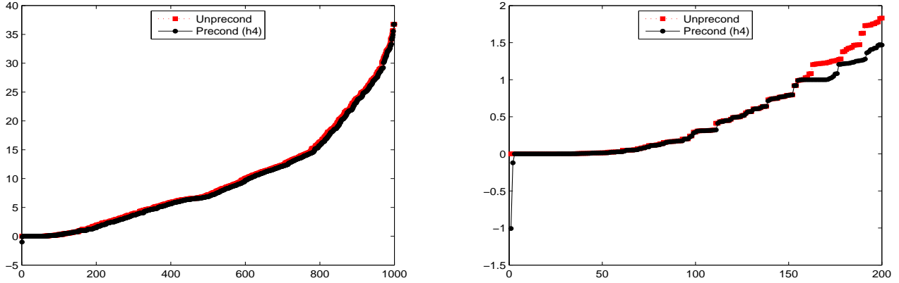
Figure 4.6: Comparison between the full spectra/detailed spectra (left figure/right figure) of \nabla^2 f(x_{k+1}) ( Unprecond ) and M_h^\sharp(0, 1, I_n)\nabla^2 f(x_{k+1}) ( Precond ), for the optimization problem NON-CVXUN, with h = h_4 = 16 . The eigenvalues in \Lambda[M_h^\sharp(0, 1, I_n)\nabla^2 f(x_{k+1})] larger than +1 are evidently scaled, so that \Lambda[M_h^\sharp(0, 1, I_n)\nabla^2 f(x_{k+1})] is more clustered.
