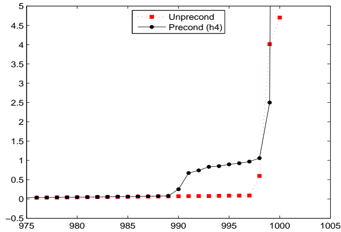
Figure 4.8: Comparison between the full spectra/detailed spectra (upper figure/lower figures) \Lambda[\nabla^2 f(x_{k+1})] ( Unprecond ) and \Lambda[M_h^\sharp(0, 1, I_n)\nabla^2 f(x_{k+1})] ( Precond ), for the optimization problem NONDQUAR, with h = h_4 = 16 . Some nearly-zero eigenvalues in the spectrum \Lambda[\nabla^2 f(x_{k+1})] are shifted to non-zero values in \Lambda[M_h^\sharp(0, 1, I_n)\nabla^2 f(x_{k+1})] . Since many eigenvalues in \Lambda[\nabla^2 f(x_{k+1})] are zero or nearly-zero, the preconditioner M_h^\sharp(0, 1, I_n) may be of scarce effect, unless large values of the parameter h are considered.
