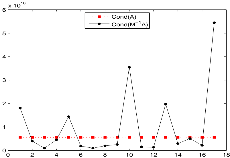
Figure 4.5: The condition number of matrix \nabla^2 f(x_{k+1}) ( Cond(A) ) along with the condition number of matrix M_h^\#(0, 1, I_n)\nabla^2 f(x_{k+1}) ( Cond(M^{-1}A) ), for the optimization problem NONCVXUN, when 1 \leq h \leq 17 . The condition number of \nabla^2 f(x_{k+1}) is nearby the condition number of M_h^\#(0, 1, I_n)\nabla^2 f(x_{k+1}) , for any value of the parameter h . The value k = 175 was chosen as in (4.3) and it was \|x_{176} - x_{175}\| \approx 0.083 .
