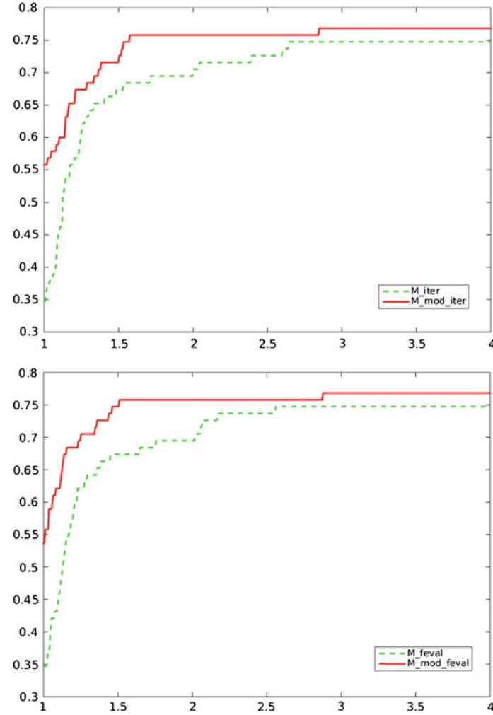
Fig. 3 Comparison between the proposal of preconditioner in (5) (namely M , dash line ) and the proposal in (7) (namely M_{\text{mod}} , solid line ), using the stopping criterion (6). Profiles with respect to # iterations (up) and # function evaluations (down)
